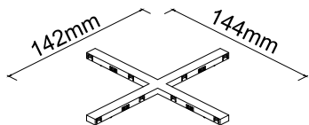
Code: LC4-11 X-90° Connector
